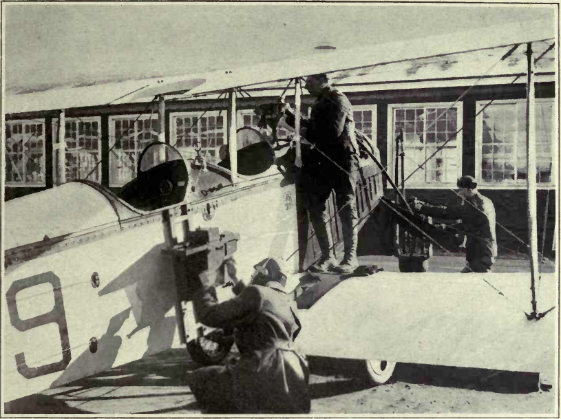
ATTACHING CAMERA TO FUSELAGE.
