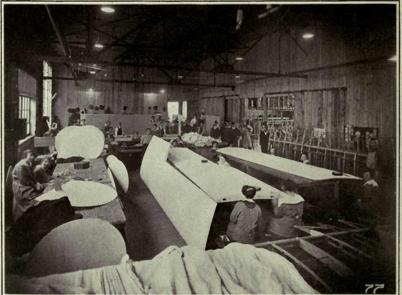
SAILMAKING ON WINGS.
