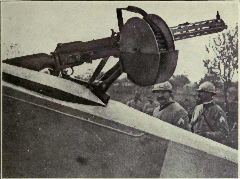
GERMAN PARABELLUM MOUNTING.
