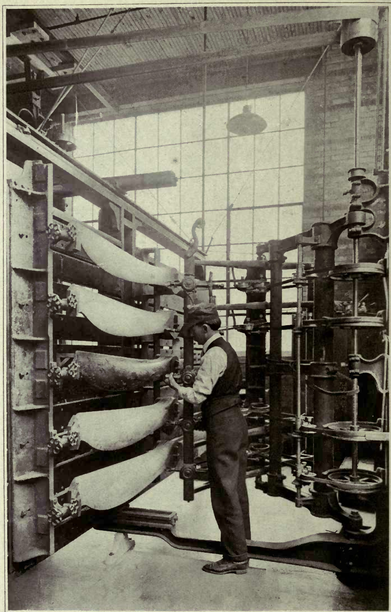
FINISHING PROPELLERS
