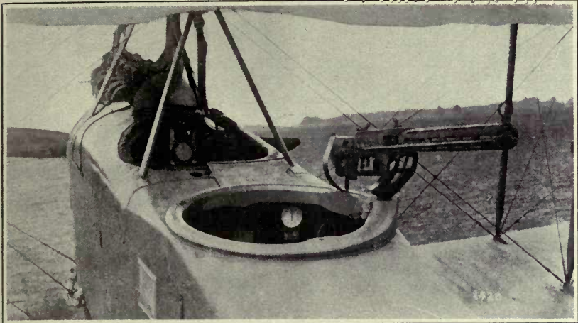
OBSERVERS' GUN MOUNTING
